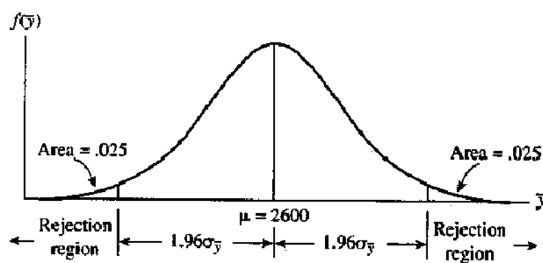
FIGURE 5.11 Rejection region for H_a : \mu \neq 2,600 when \alpha = .05
